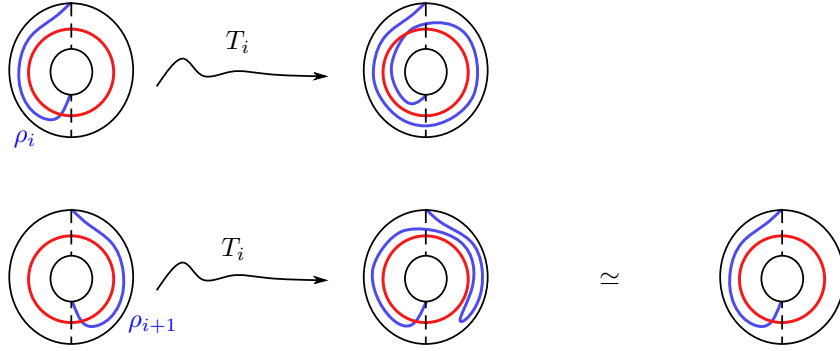
FIGURE 7. The action of the Dehn twist T_i on the arcs \rho_i (top) and \rho_{i+1} (bottom)
