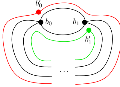
FIGURE 2. Regular bad 1-simplex with \nu = 1 .
