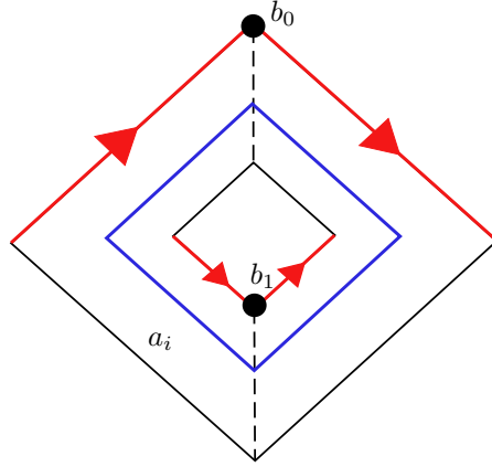
FIGURE 4. The curve a_i in D_i \# D_{i+1}
