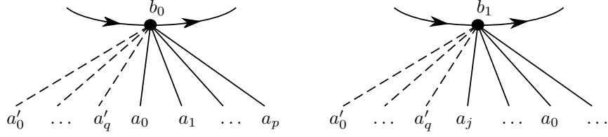
FIGURE 1. Maximal regular bad simplex \{a_0, \dots, a_p\} and simplex \{a'_0, \dots, a'_q\} in its link.
