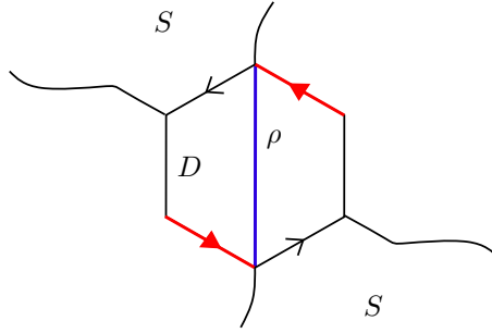
FIGURE 8. Cutting along the core of a disk
